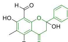
84 R 1 = OMe 85 R 1 = OH
