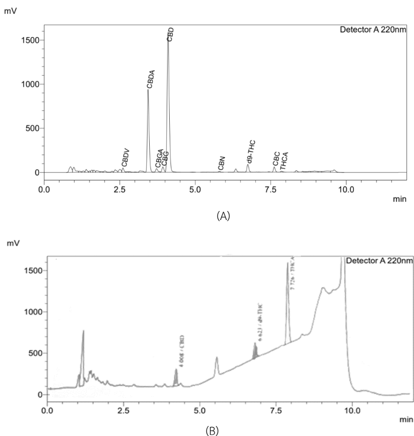
Figure 3 HPLC-UV chromatogram of (A) Cannabis sp. "Charlotte's angel" detection at 220 nm. The compounds elute in the following order: CBD-acid (tR: 3.442 min), CBD (tR: 4.100 min), CBN (tR: 5.801 min), THC (tR: 6.741 min), THC-acid A (tR: 7.858 min) (B) Cannabis sp. Thai stick "Phuphan"
