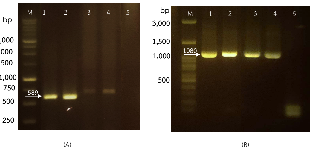
Figure 2 PCR results for (A) active THCA band (B) active CBDA band
