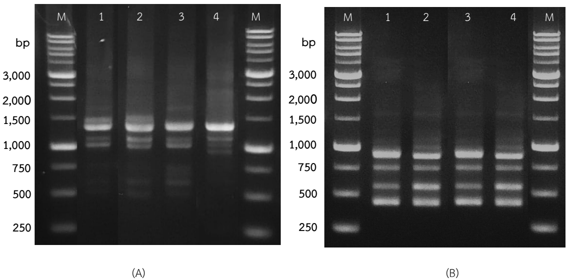
Figure 5 Result of gel electrophoresis of PCR products obtained by using (A OPA-10, B OPH-17) RAPD primer Lane M: marker, 1: Cannabis sp. Thai stick “Phuphan”, 2-4 callus of Cannabis sp. Thai stick “Phuphan”
