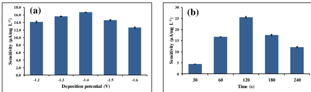
Figure 2. The effect of preconcentration potential (a) and The effect of preconcentration time (b) on the sensitivity of Zn(II) on the Bi/poly(L-cys). The sensitivity is slope of the calibration curve at the concentration of Zn(II) between 0.05 and 0.50 mg L -1 . (ASV operation conditions: 60 s preconcentration time, -1.40 V preconcentration potential with stirring, square-wave potential scan between -1.40 and -0.50 V).
