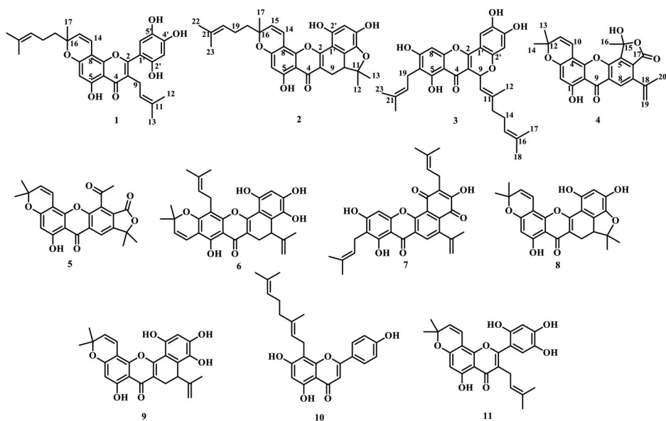
Figure 1. The structures of compounds 1–11.
